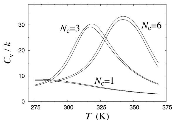
FIGURE 4 Specific heat C_v against temperature T for N_c = 1, 3 , and 6 A \beta_{16-22} peptides, as obtained using histogram reweighting techniques (Ferrenberg and Swendsen, 1988). The bands are centered around the expected values and show statistical 1\sigma errors. C_v is defined as C_v = (N_c N)^{-1} d\langle E \rangle / dT = (N_c N k T^2)^{-1} (\langle E^2 \rangle - \langle E \rangle^2) , where N_c is the number of chains, N is the number of amino acids per chain, and \langle \rangle denotes a Boltzmann average of variable O .
